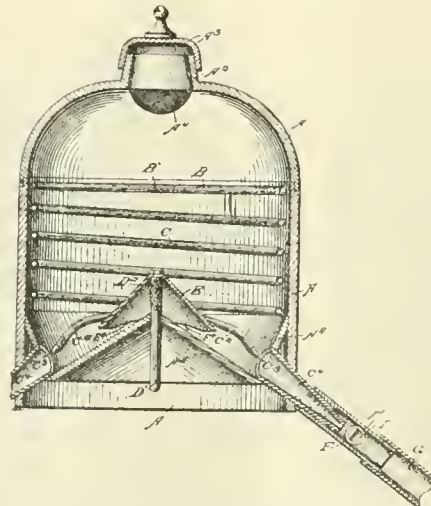
SAND BOX FOR USING WET SAND.
